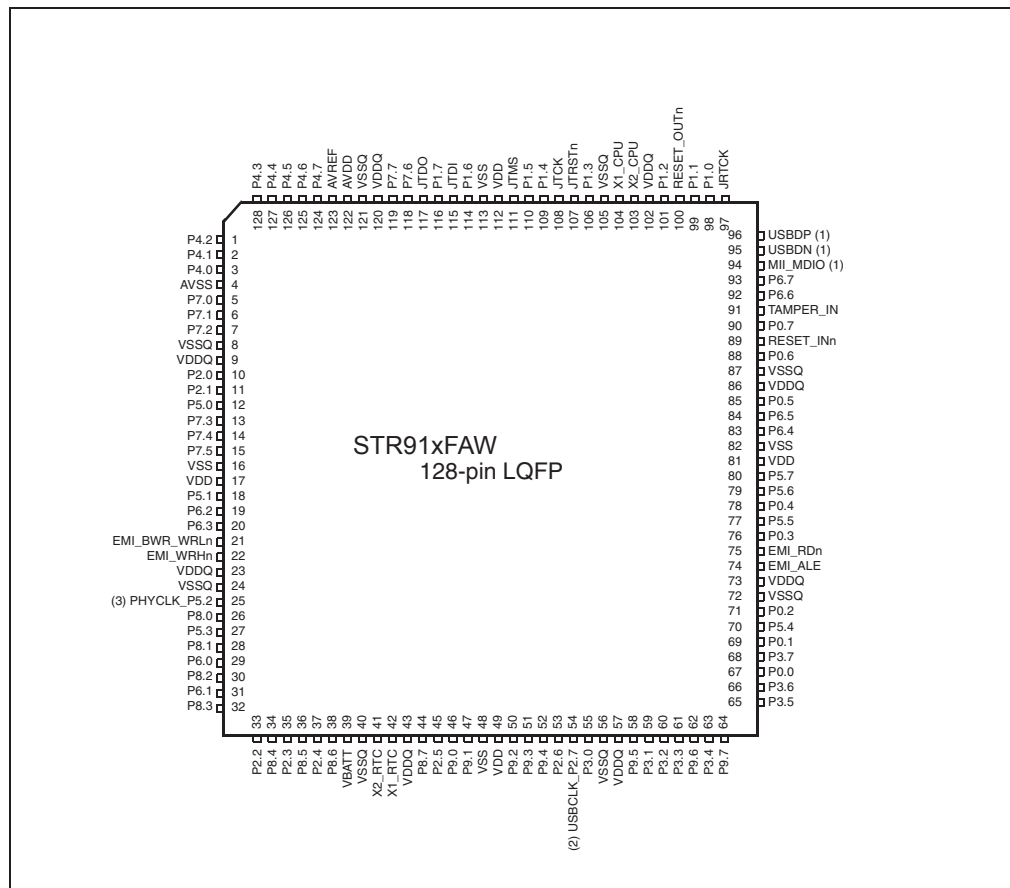
Figure 8. STR91xFAW 128-pin package pinout
