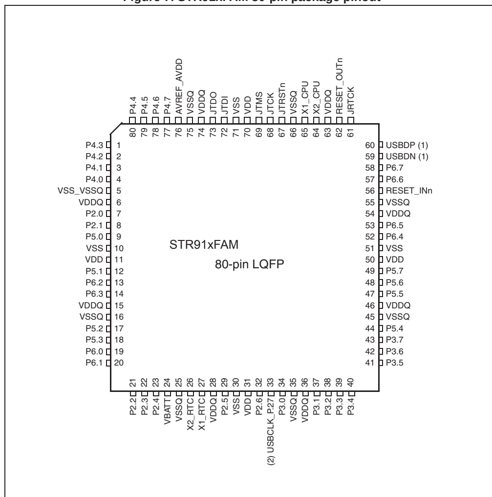
Figure 7. STR91xFAM 80-pin package pinout
